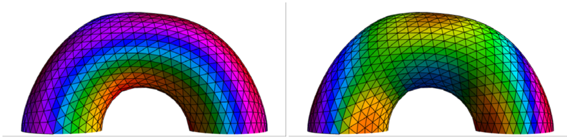
Figure: Facets in a Loop mesh colored based on their volume contribution \text{vol}(f) . Left uses the alternating forms \hat{Y}^{\tau(f)} , and right visualizes the difference Y^{\tau(f)} - \hat{Y}^{\tau(f)} . ■
