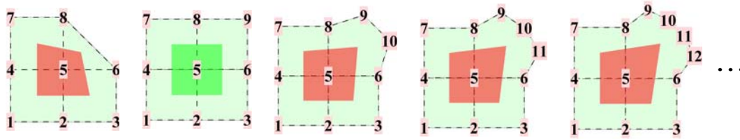
Figure: Facets of a Doo-Sabin mesh with \tau(f) \in \{3, 4, \dots, 7\} , and m(f) \in \{8, 9, \dots, 12\} , and indexing of the control points. ■
