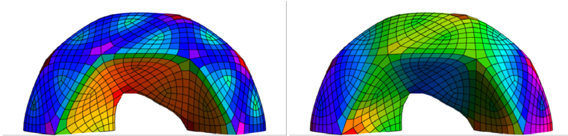
Figure: Facets of a Catmull-Clark mesh colored based on their volume contribution \text{vol}(f) . Left uses the alternating forms \hat{Y}^{\tau(f)} , and right visualizes the difference \bar{Y}^{\tau(f)} - \hat{Y}^{\tau(f)} . ■
