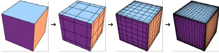
Figure: 3 rounds of Catmull-Clark subdivision of the degenerate mesh. ■
