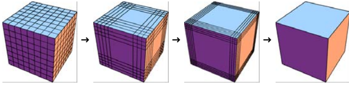
Figure: Construction of the degenerate cube mesh M : Linear subdivision followed by vertex collapse. ■
