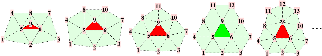
Figure: Indexing of vertices in the one-ring of a triangular facet f for \tau(f) \in \{3, 4, 5, 6, 7\} . ■
