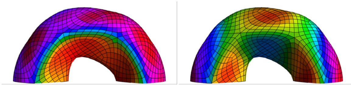
Figure: Facets of a Doo-Sabin mesh colored based on their volume contribution \text{vol}(f) . Left uses the alternating forms \hat{Y}^{\tau(f)} , and right visualizes the difference \bar{Y}^{\tau(f)} - \hat{Y}^{\tau(f)} . ■
