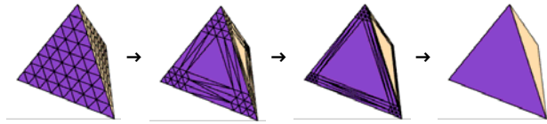
Figure: The construction of the degenerate mesh M : Linear subdivision followed by vertex collapse. ■
